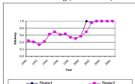
Graph 8: Technical Efficiency with(out) inflation accounting (State Banks)
