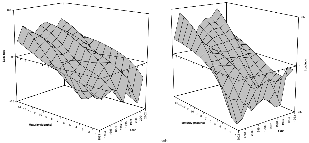
Figure 6: Rotated loadings on factor 2 on January for two year windows
